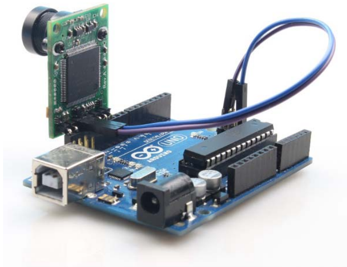
Figure 2 Wiring for Arduino UNO R3
