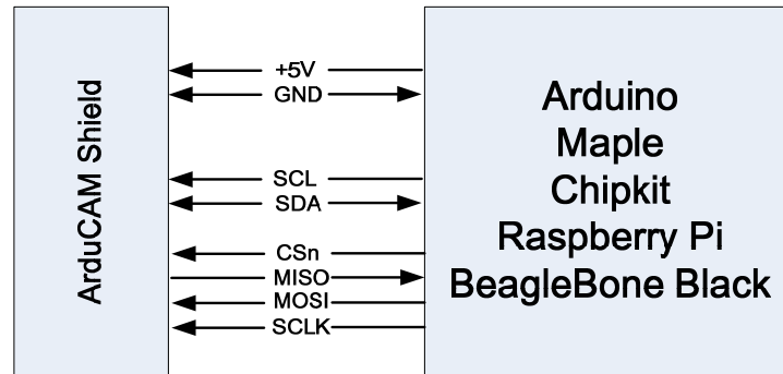
Figure 1 Typical Wiring
