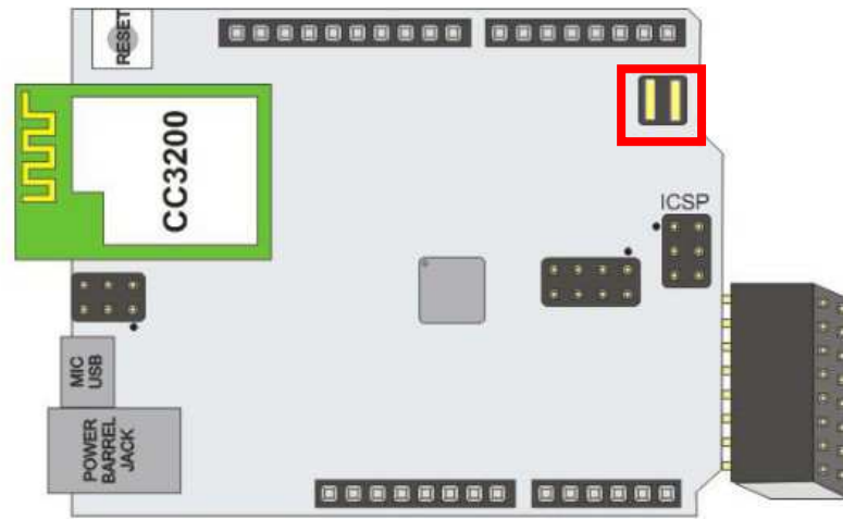
Figure 3 Jumper Connection for Energia
